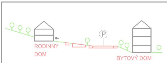
REZ E-E'
